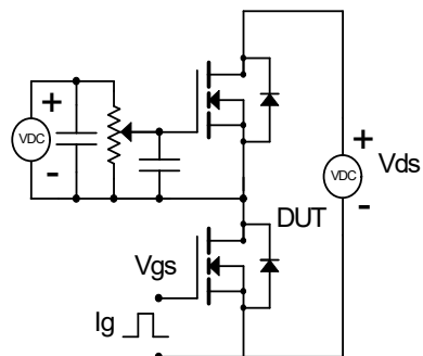
Gate Charge Test Circuit & Waveform
